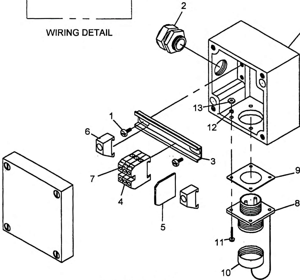
EXPLODED VIEW
