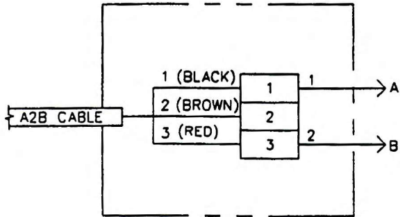
WIRING DETAIL
